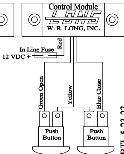
Wiring Diagram using two Push Buttons in Handle
