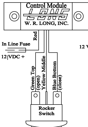
Wiring Diagram for Rocker Switch in Handle
